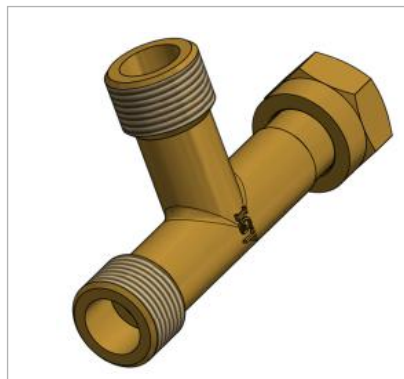
T- connection for second cylinder attachment.
