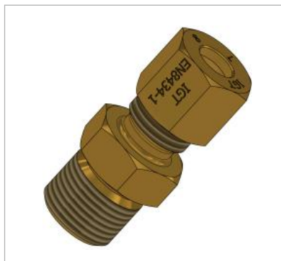
Nut entry 8 mm compression fitting Exits G3/8 LH male Reference A900-364
