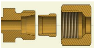
Compression fitting to EN8434
